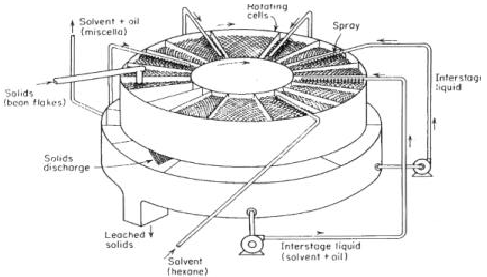
Rotocell or Carousel Extractor
